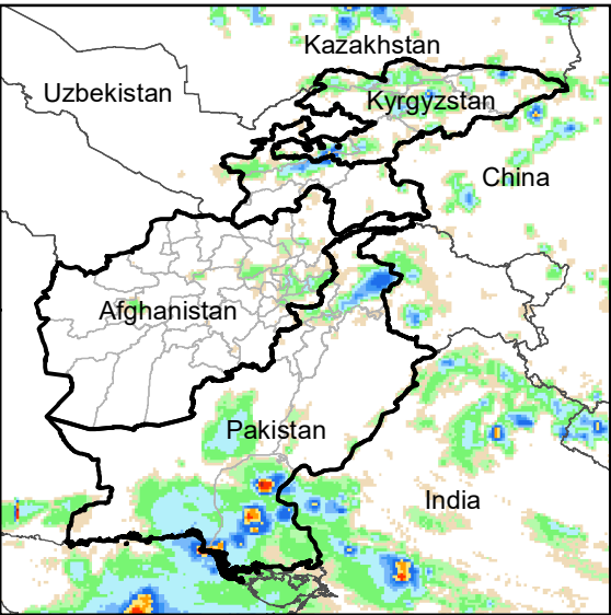
Daily Rainfall estimate for 20 Jul., 2020
