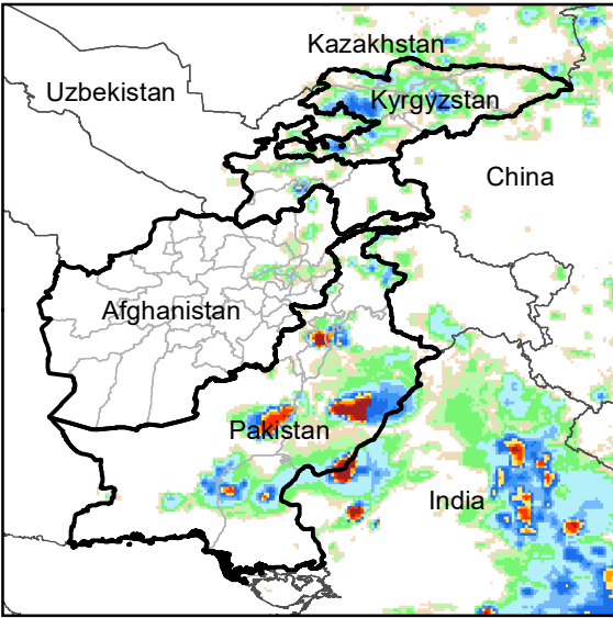
Daily Rainfall estimate for 21 Jul., 2020
