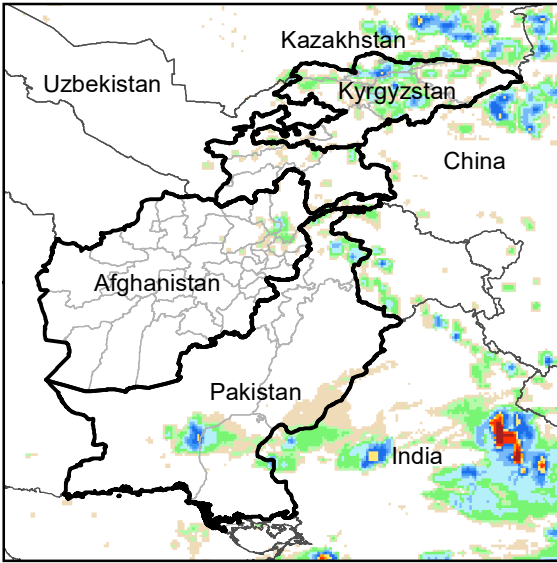
Daily Rainfall estimate for 22 Jul., 2020
