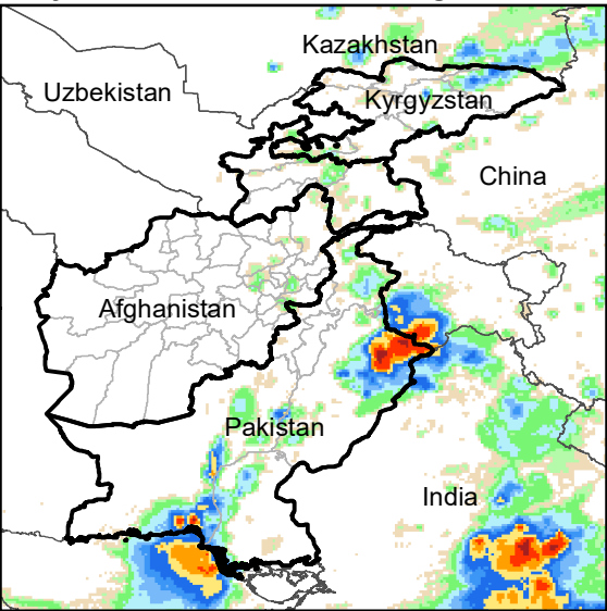
Daily Rainfall estimate for 30 Aug., 2020
