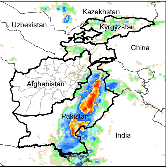
Daily Rainfall estimate for 31 Aug., 2020
