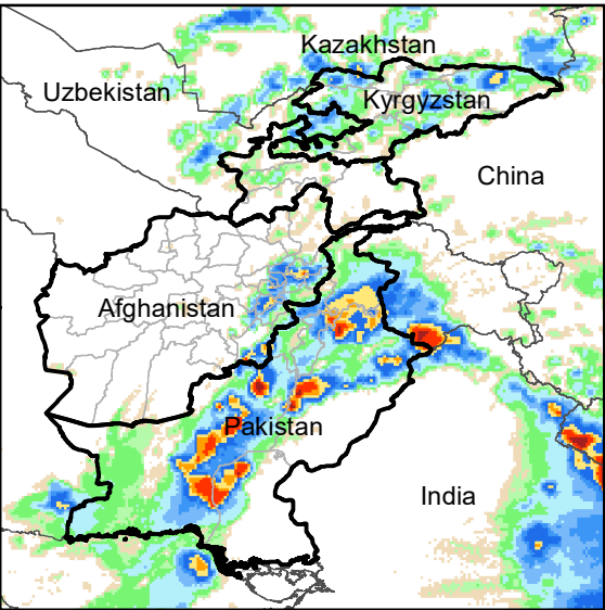
Daily Rainfall estimate for 29 Aug., 2020
