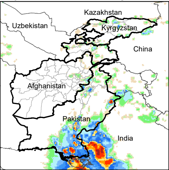
Daily Rainfall estimate for 2 Sep., 2020
