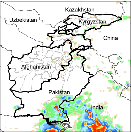
Daily Rainfall estimate for 1 Sep., 2020
