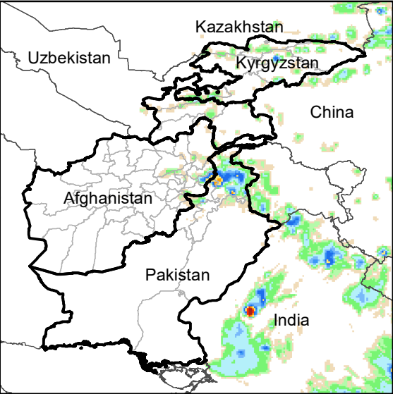
Daily Rainfall estimate for 9 Sep., 2020
