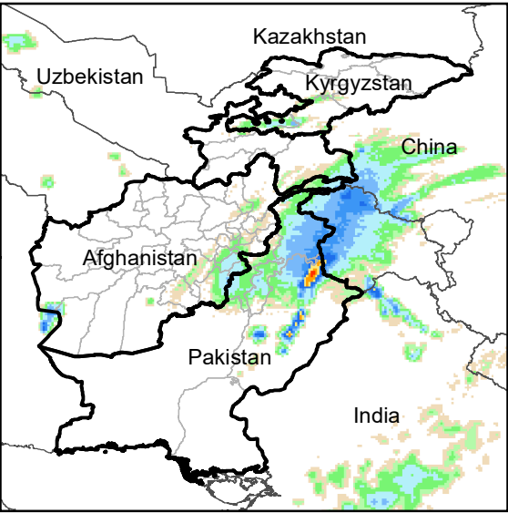
Daily Rainfall estimate for 11 Dec., 2020
