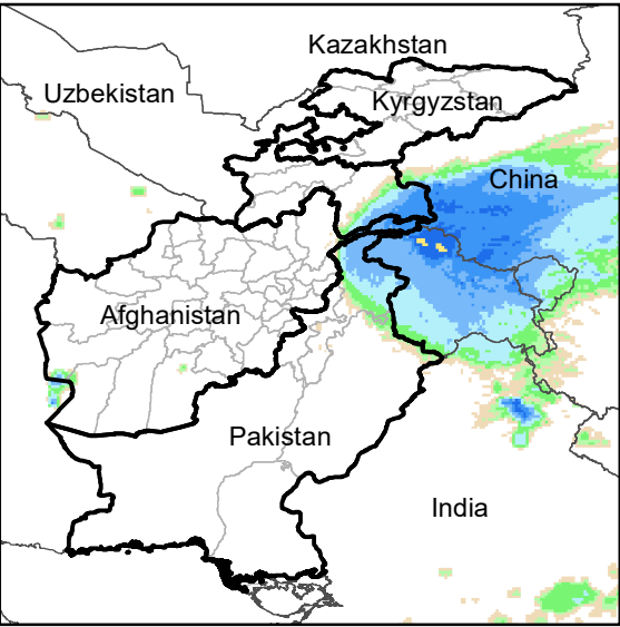
Daily Rainfall estimate for 12 Dec., 2020
