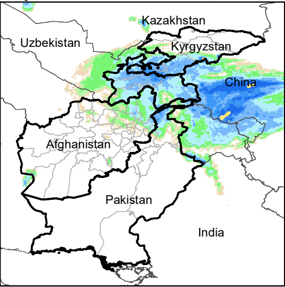
Daily Rainfall estimate for 27 Dec., 2020
