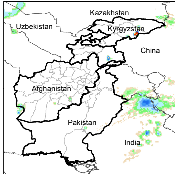
Daily Rainfall estimate for 2 Jan., 2021
