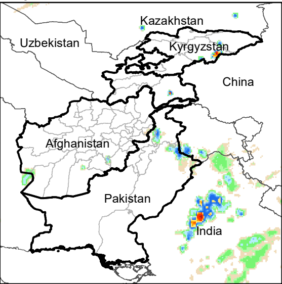
Daily Rainfall estimate for 7 Jan., 2021
