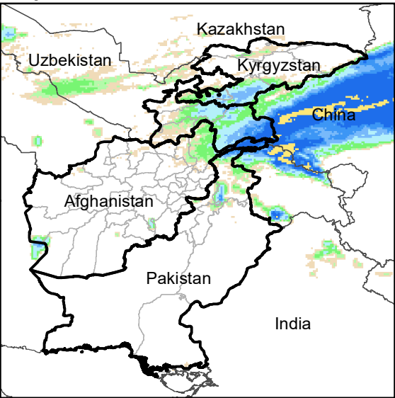
Daily Rainfall estimate for 1 Mar., 2021
