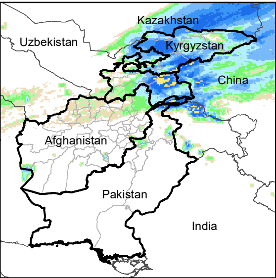
Daily Rainfall estimate for 28 Feb., 2021
