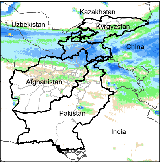
Daily Rainfall estimate for 19 Mar., 2021
