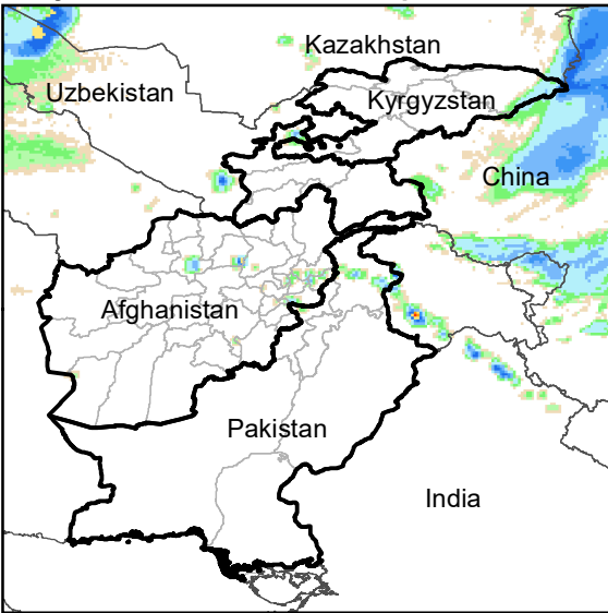
Daily Rainfall estimate for 5 Apr., 2021
