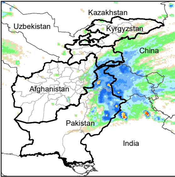
Daily Rainfall estimate for 6 Apr., 2021
