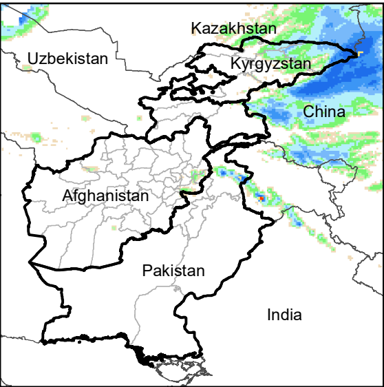
Daily Rainfall estimate for 4 Apr., 2021
