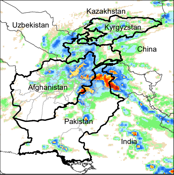
Daily Rainfall estimate for 10 May., 2021
