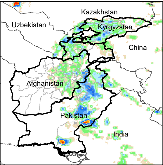
Daily Rainfall estimate for 25 May., 2021
