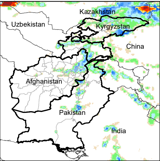
Daily Rainfall estimate for 31 May., 2021
