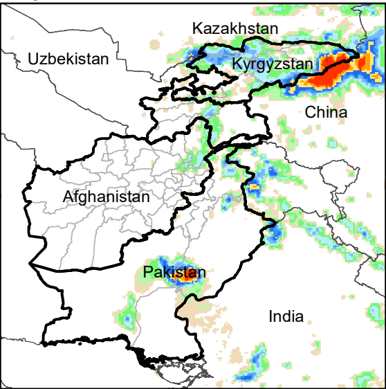
Daily Rainfall estimate for 6 Jun., 2021
