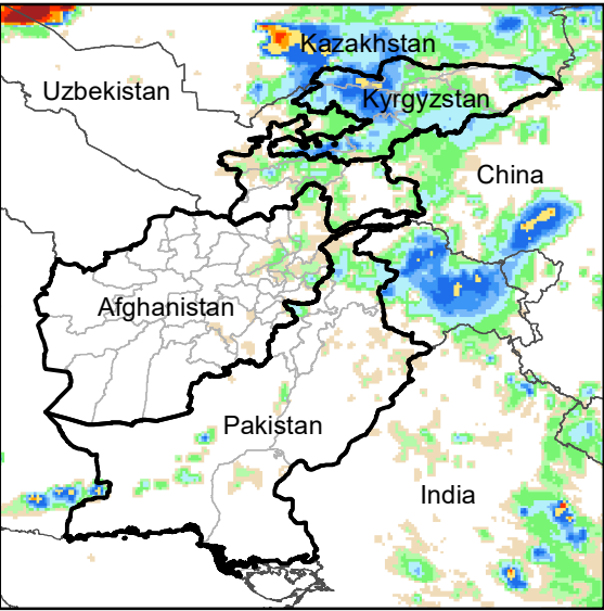
Daily Rainfall estimate for 6 Jul., 2021
