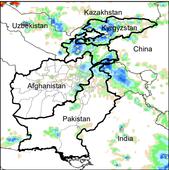
Daily Rainfall estimate for 8 Jul., 2021
