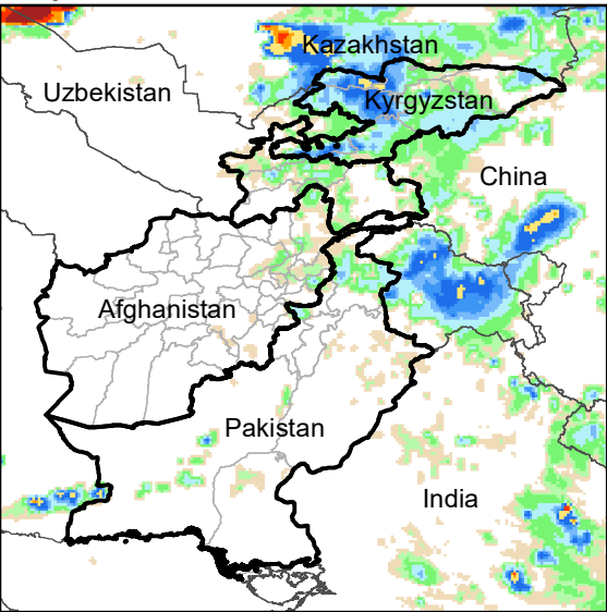
Daily Rainfall estimate for 9 Jul., 2021
