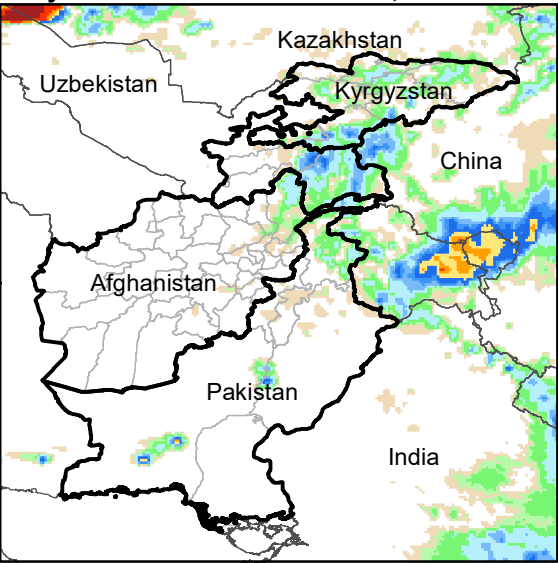
Daily Rainfall estimate for 7 Jul., 2021
