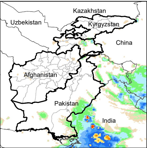
Daily Rainfall estimate for 28 Jul., 2021
