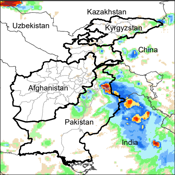
Daily Rainfall estimate for 31 Jul., 2021
