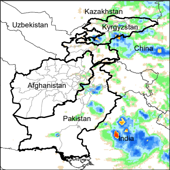
Daily Rainfall estimate for 2 Aug., 2021
