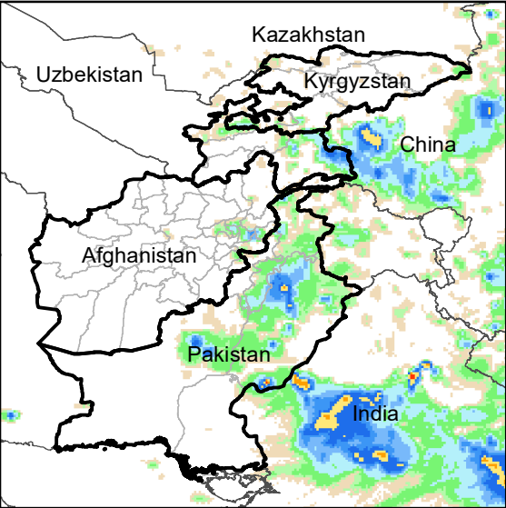
Daily Rainfall estimate for 3 Aug., 2021
