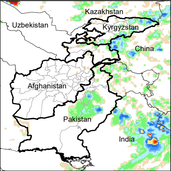
Daily Rainfall estimate for 1 Aug., 2021
