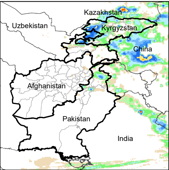
Daily Rainfall estimate for 16 Aug., 2021
