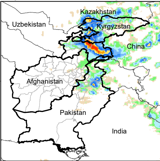
Daily Rainfall estimate for 17 Aug., 2021
