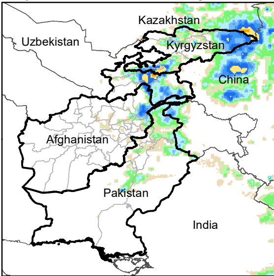
Daily Rainfall estimate for 18 Aug., 2021
