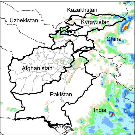
Daily Rainfall estimate for 22 Aug., 2021
