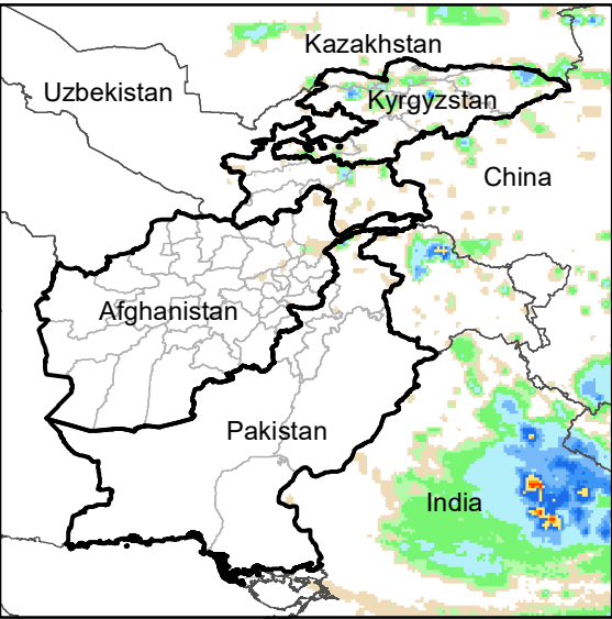
Daily Rainfall estimate for 24 Aug., 2021
