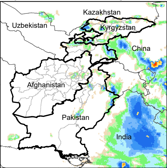
Daily Rainfall estimate for 23 Aug., 2021
