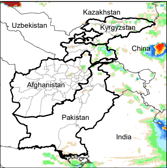
Daily Rainfall estimate for 29 Aug., 2021
