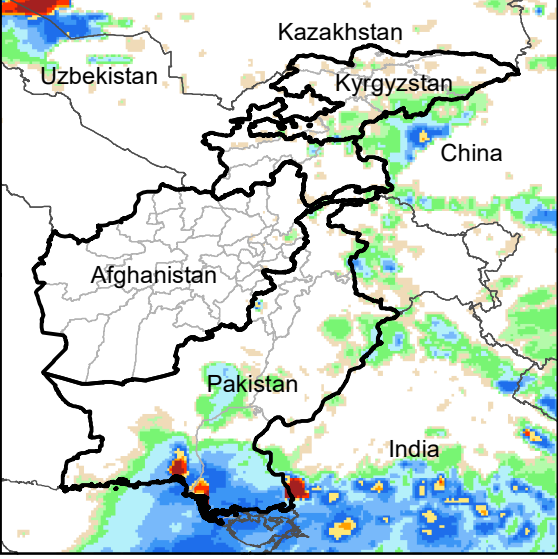
Daily Rainfall estimate for 9 Sep., 2021
