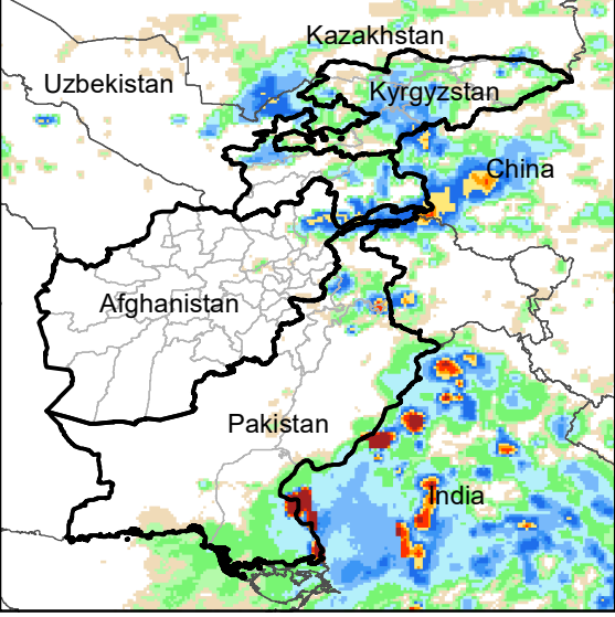
Daily Rainfall estimate for 10 Sep., 2021
