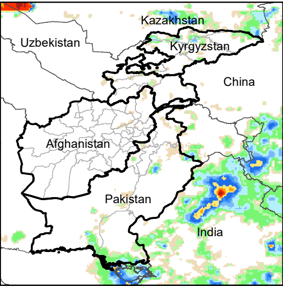
Daily Rainfall estimate for 23 Sep., 2021
