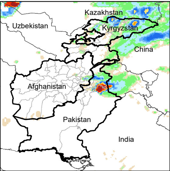
Daily Rainfall estimate for 13 Oct., 2021
