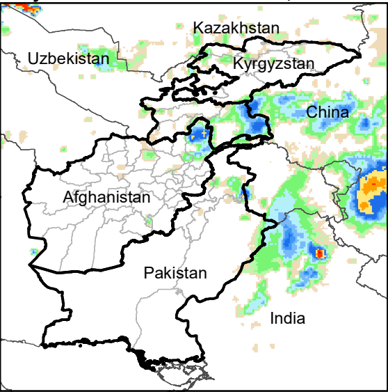
Daily Rainfall estimate for 24 Oct., 2021
