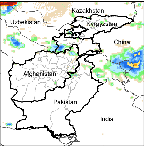
Daily Rainfall estimate for 29 Oct., 2021
