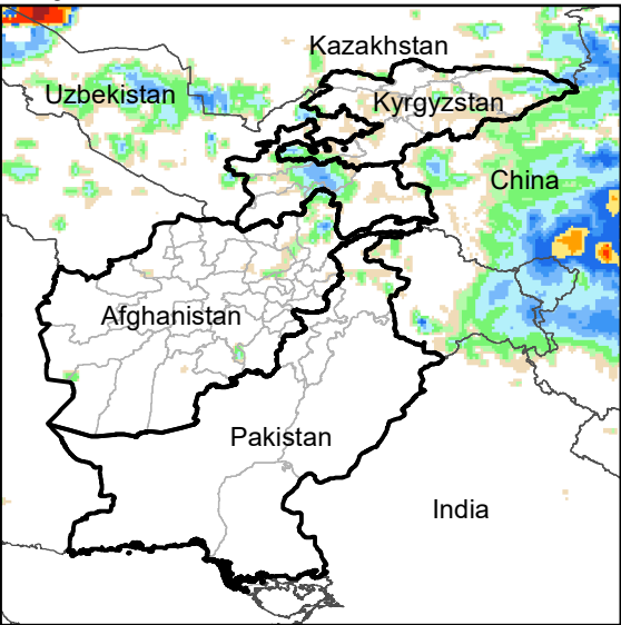
Daily Rainfall estimate for 28 Oct., 2021
