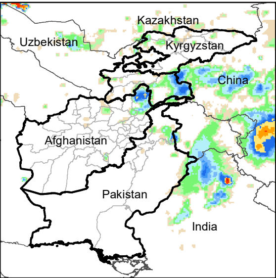
Daily Rainfall estimate for 27 Oct., 2021
