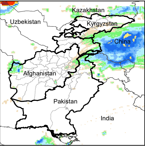
Daily Rainfall estimate for 5 Nov., 2021
