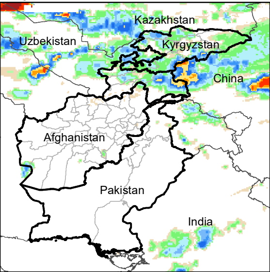
Daily Rainfall estimate for 21 Nov., 2021
