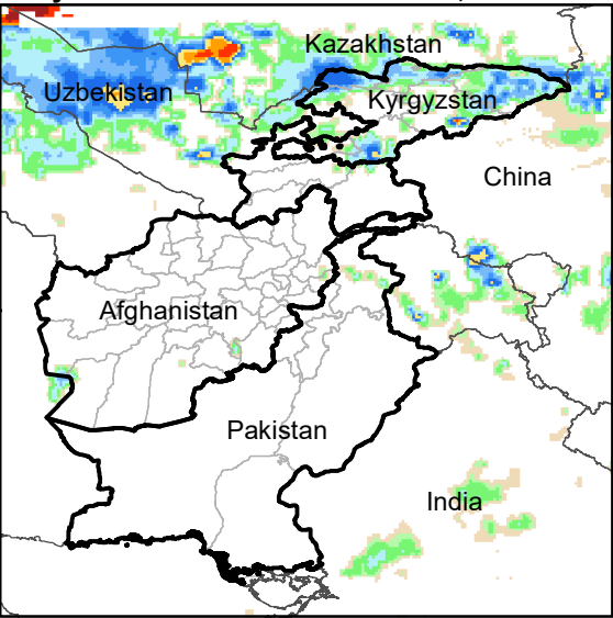
Daily Rainfall estimate for 19 Nov., 2021
