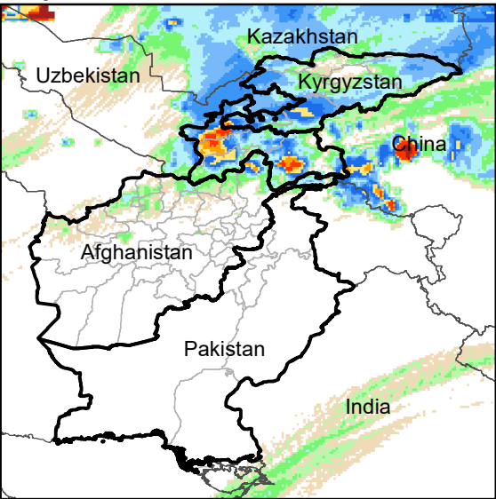
Daily Rainfall estimate for 20 Nov., 2021
