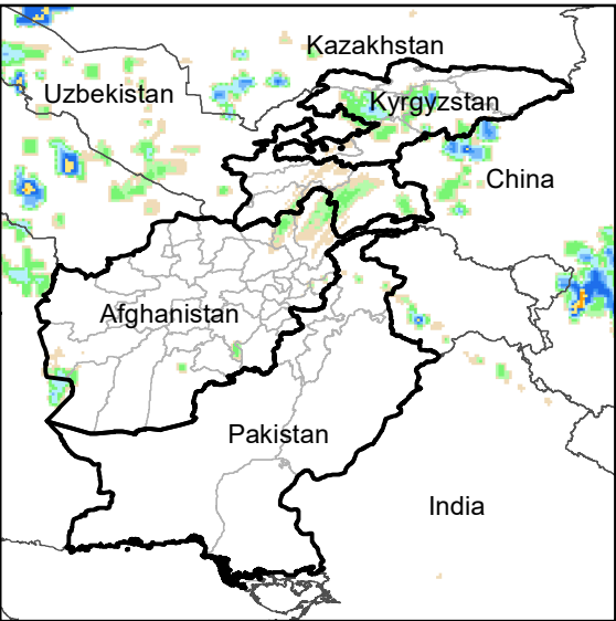
Daily Rainfall estimate for 1 Dec., 2021
