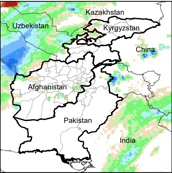
Daily Rainfall estimate for 2 Dec., 2021
