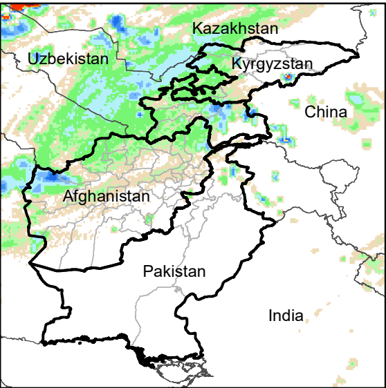
Daily Rainfall estimate for 6 Dec., 2021
