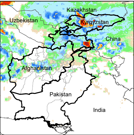
Daily Rainfall estimate for 22 Jan., 2022
