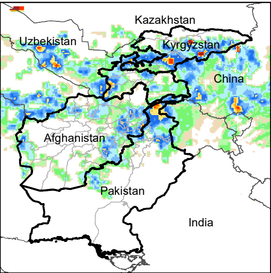
Daily Rainfall estimate for 27 Jan., 2022
