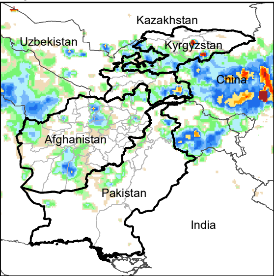
Daily Rainfall estimate for 28 Jan., 2022
