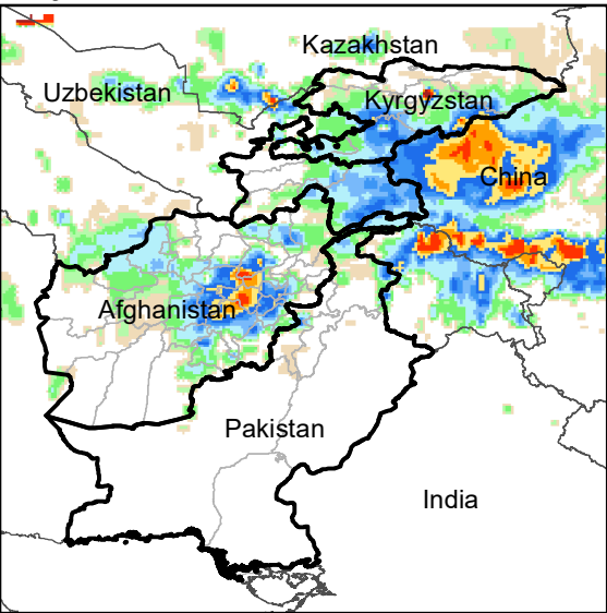
Daily Rainfall estimate for 29 Jan., 2022
