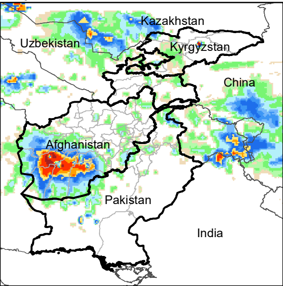
Daily Rainfall estimate for 20 Feb., 2022
