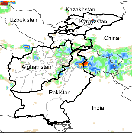
Daily Rainfall estimate for 19 Feb., 2022
