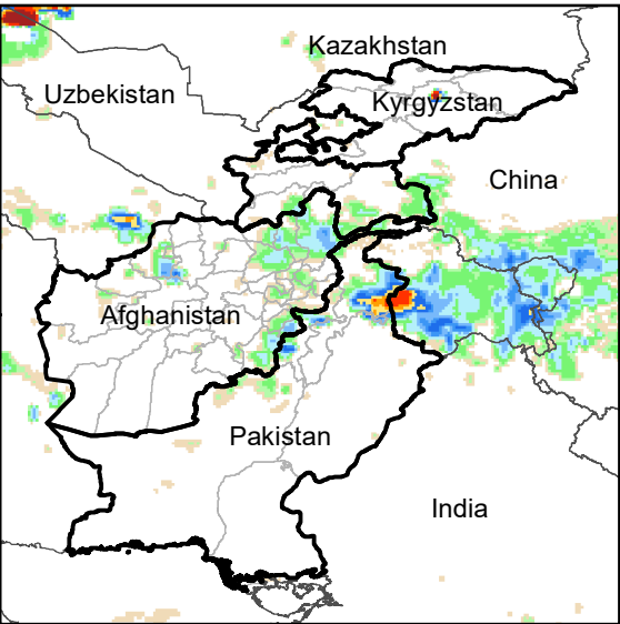
Daily Rainfall estimate for 22 Feb., 2022
