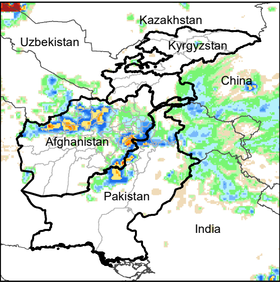
Daily Rainfall estimate for 26 Feb., 2022
