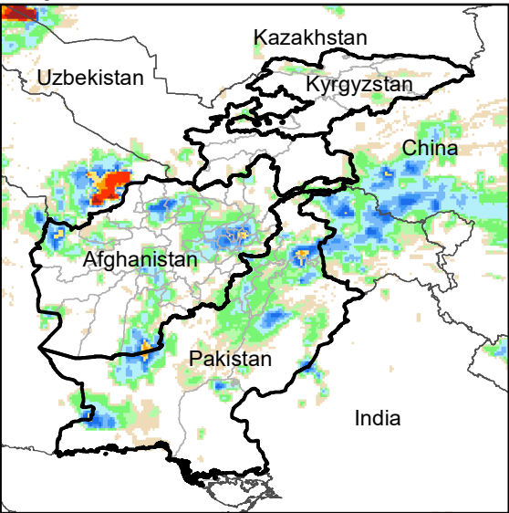
Daily Rainfall estimate for 5 Mar., 2022
