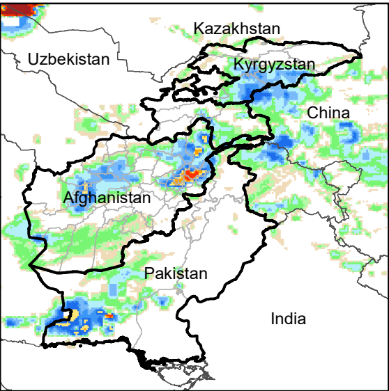
Daily Rainfall estimate for 4 Mar., 2022
