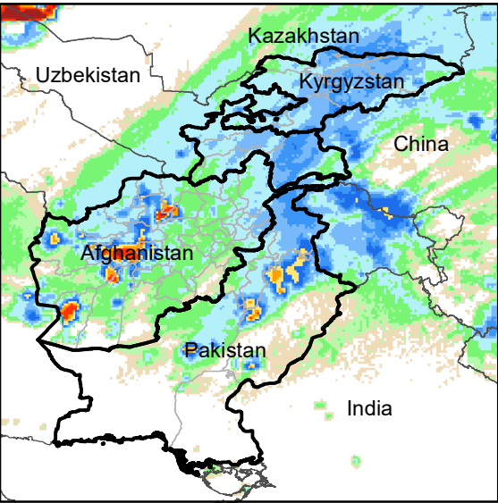
Daily Rainfall estimate for 6 Mar., 2022
