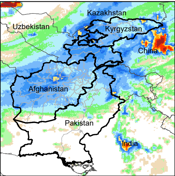
Daily Rainfall estimate for 10 Mar., 2022
