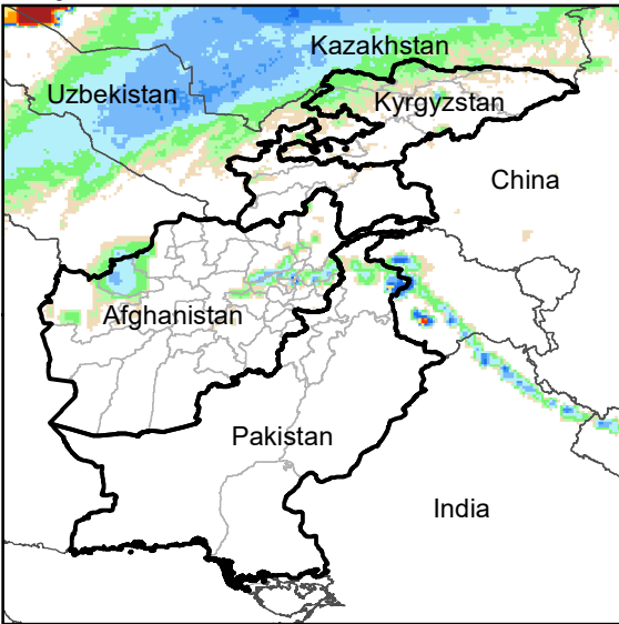
Daily Rainfall estimate for 20 Mar., 2022
