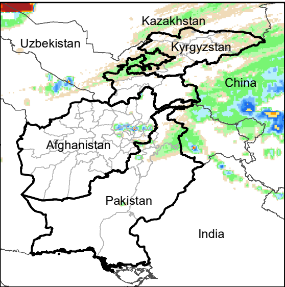
Daily Rainfall estimate for 22 Mar., 2022
