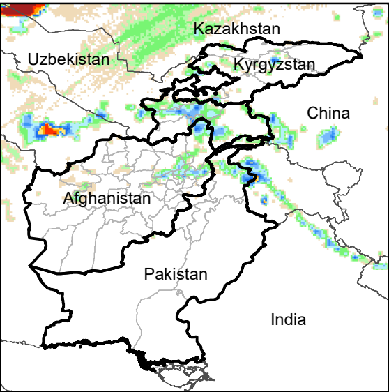
Daily Rainfall estimate for 4 Apr., 2022
