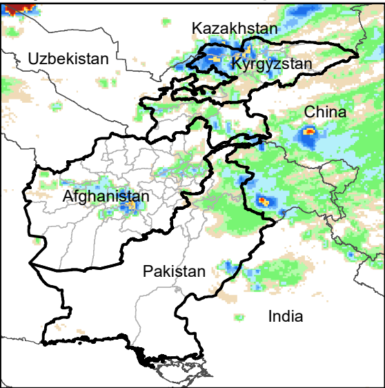
Daily Rainfall estimate for 28 Apr., 2022
