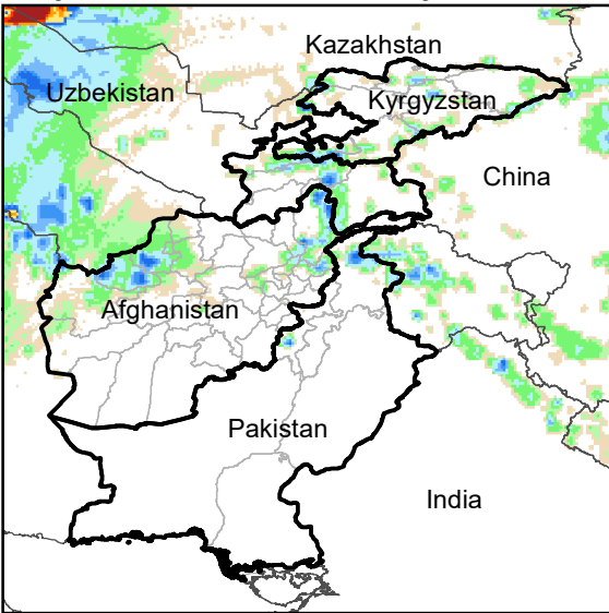
Daily Rainfall estimate for 11 May., 2022
