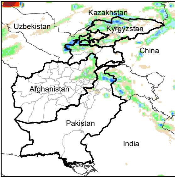
Daily Rainfall estimate for 12 May., 2022
