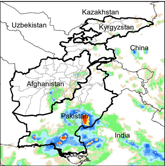
Daily Rainfall estimate for 16 Aug., 2022
