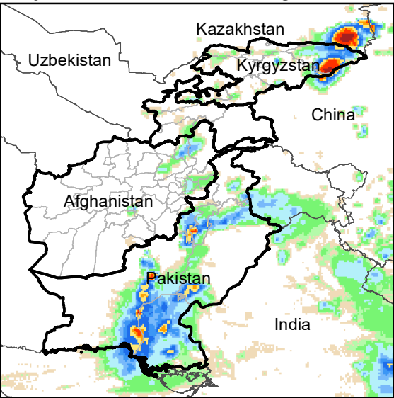
Daily Rainfall estimate for 27 Aug., 2022
