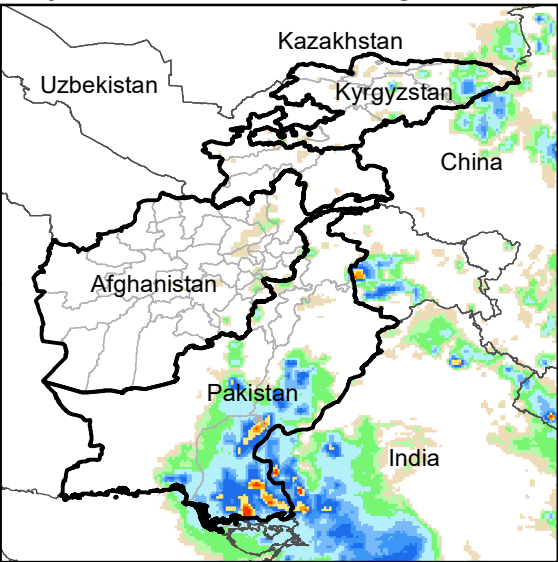
Daily Rainfall estimate for 26 Aug., 2022
