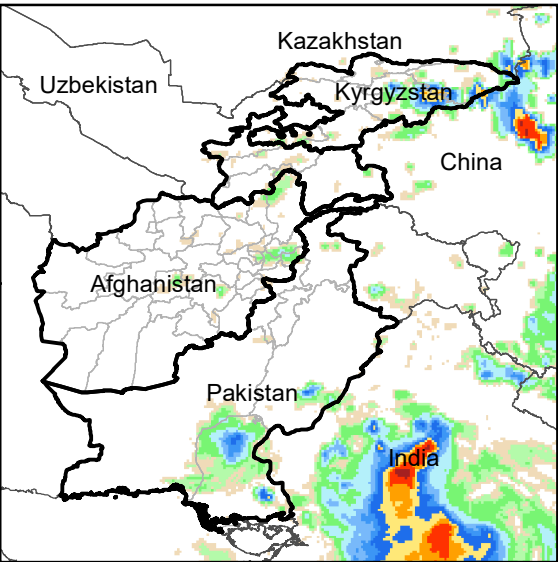
Daily Rainfall estimate for 25 Aug., 2022
