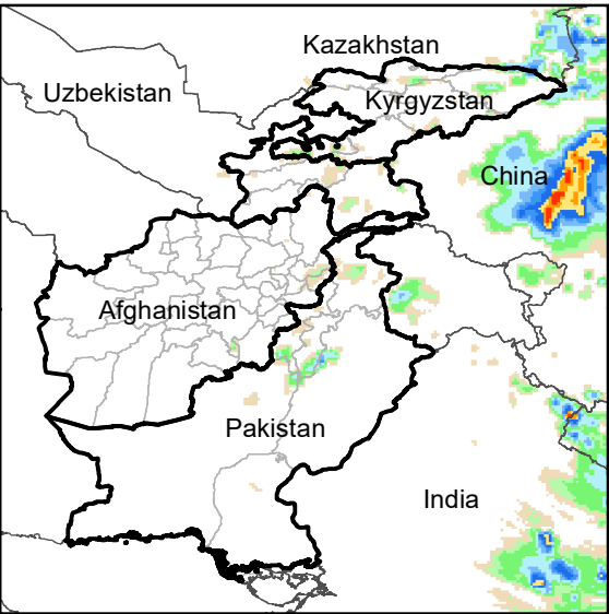
Daily Rainfall estimate for 30 Aug., 2022
