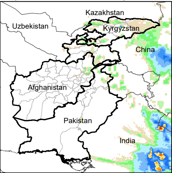
Daily Rainfall estimate for 31 Aug., 2022
