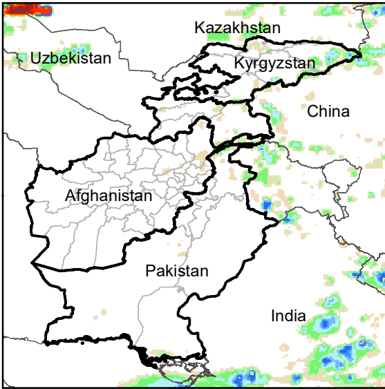
Daily Rainfall estimate for 9 Sep., 2022
