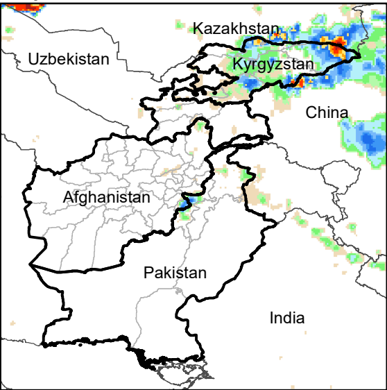
Daily Rainfall estimate for 5 Oct., 2022
