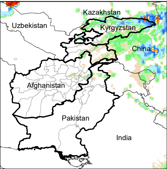
Daily Rainfall estimate for 6 Oct., 2022
