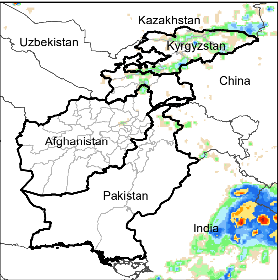
Daily Rainfall estimate for 12 Oct., 2022
